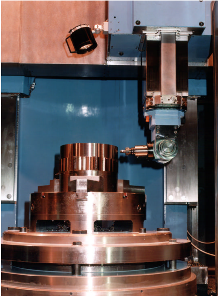
Right Angle and Adjustable Angle Heads Installed on a Millennium Machine for Installation Trials at WEBSTER & BENNETT Factory, COVENTRY, UK. Final customer – KAISER, USA.
